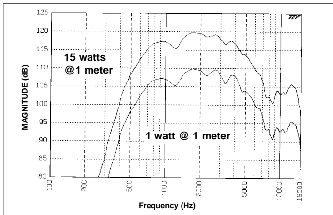
AP-15(T) Frequency Response
