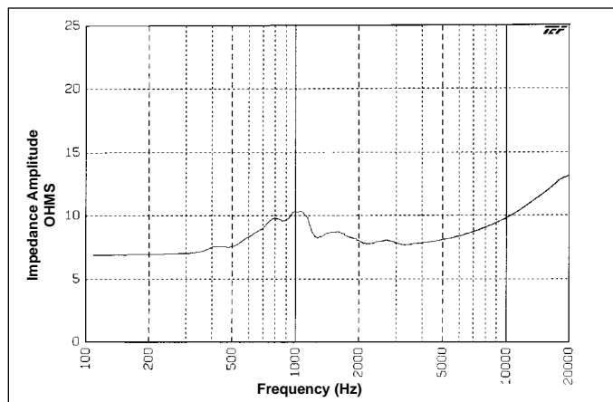
AP-15 (Impedance Sweep)
