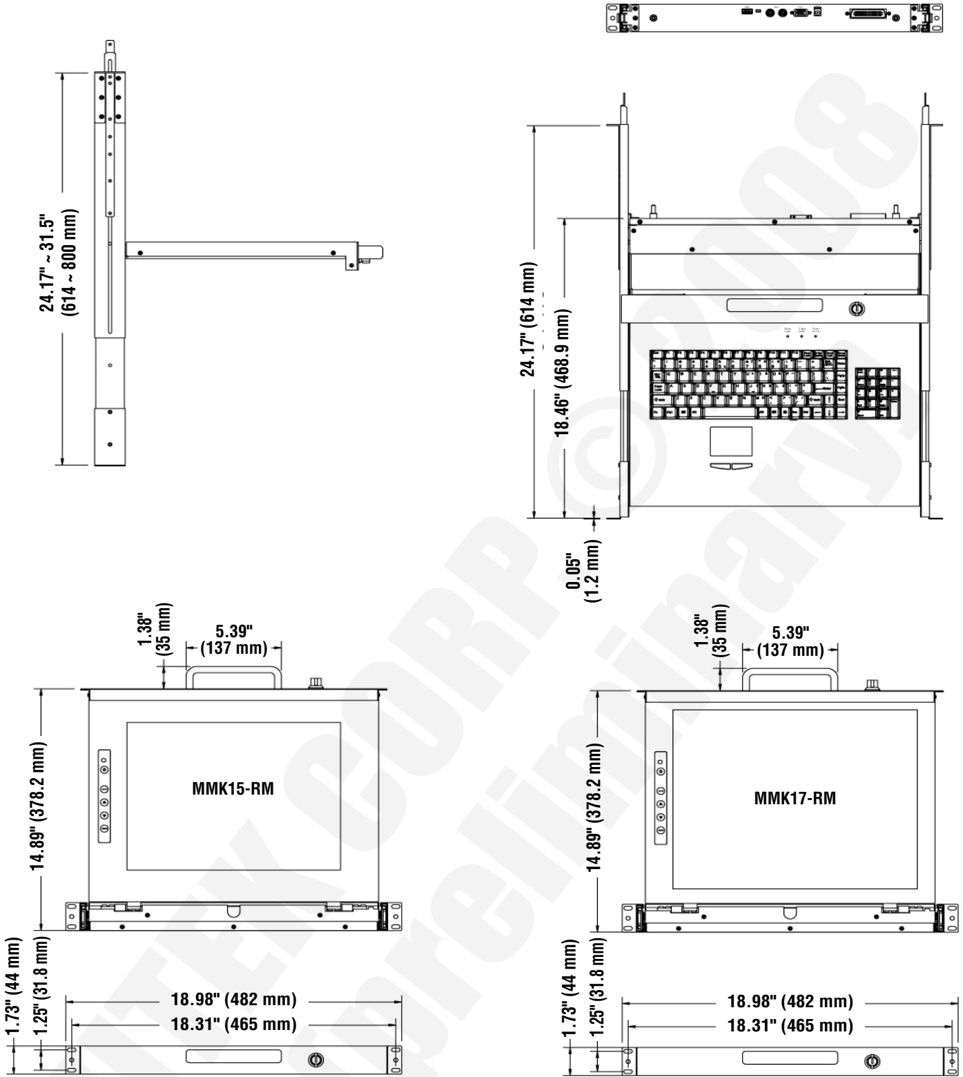
15" / 17" Single Rail Console with Modular KVM Switch Dimensions
